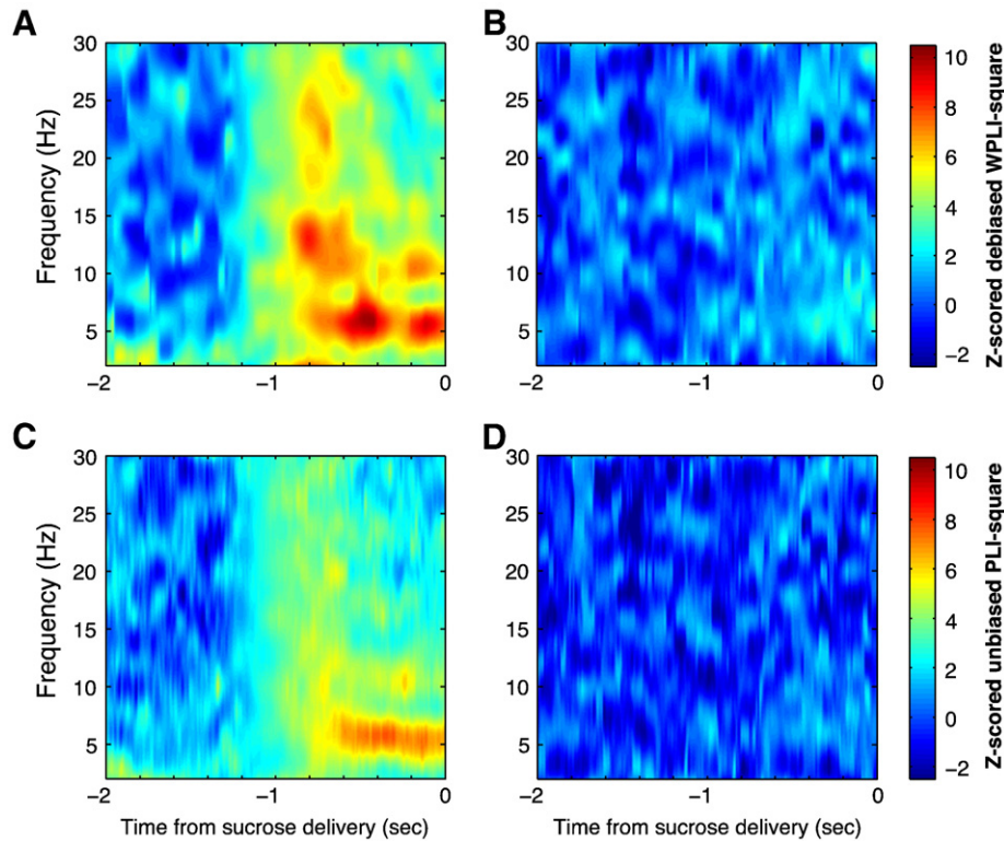
Fig. 13. Comparison of z-scored debiased WPLI-square estimator and z-scored unbiased PLI-square estimator. All figures have same color scaling to enhance comparability. (A) Average z-score standardized debiased WPLI-square estimator as function of time and frequency during the correct go waiting (for sucrose) period. (B) Average z-score standardized debiased WPLI-square estimator as function of time and frequency during the incorrect go waiting (for quinine) period. (C) Average z-score standardized unbiased PLI-square estimator as function of time and frequency during the correct go waiting (for sucrose) period. (D) Average z-score standardized unbiased PLI-square estimator as function of time and frequency during the incorrect go waiting (for quinine) period.
